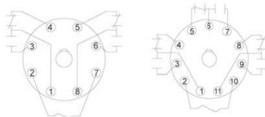
DPDT
